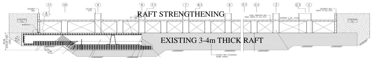
Figure 2 – Raft Strengthening Section (TTW) 筏结构横截面
