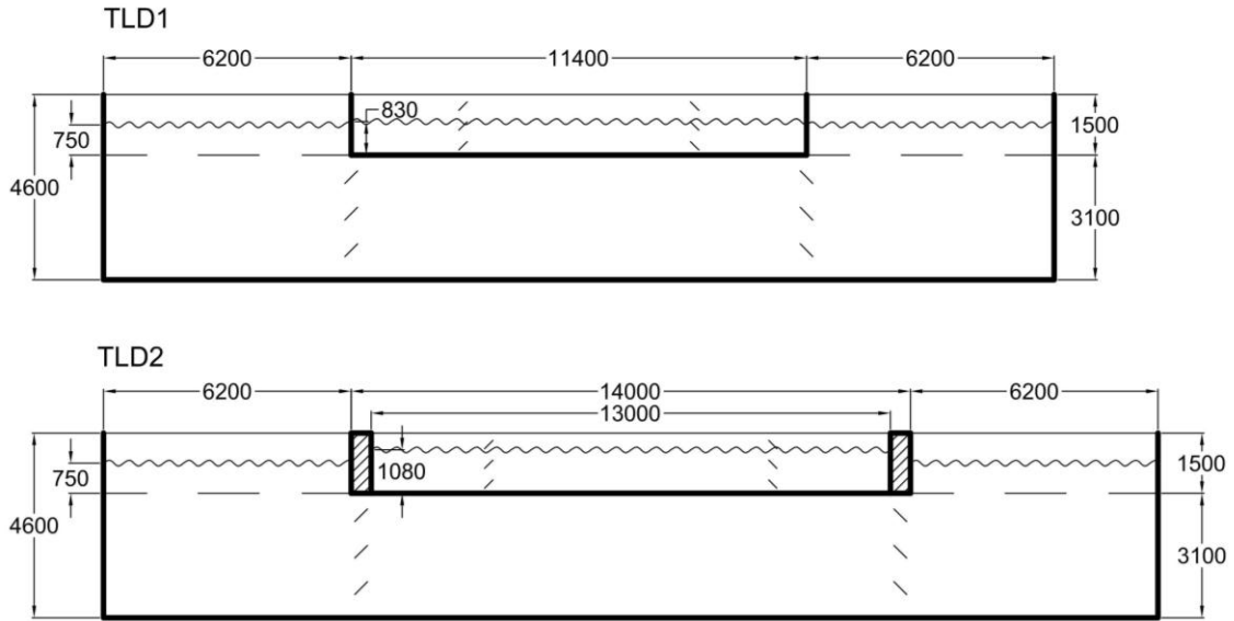
(b) Section Views for the two Tuned Liquid Dampers on Level 44. 两个调谐液体阻尼器的截面图
