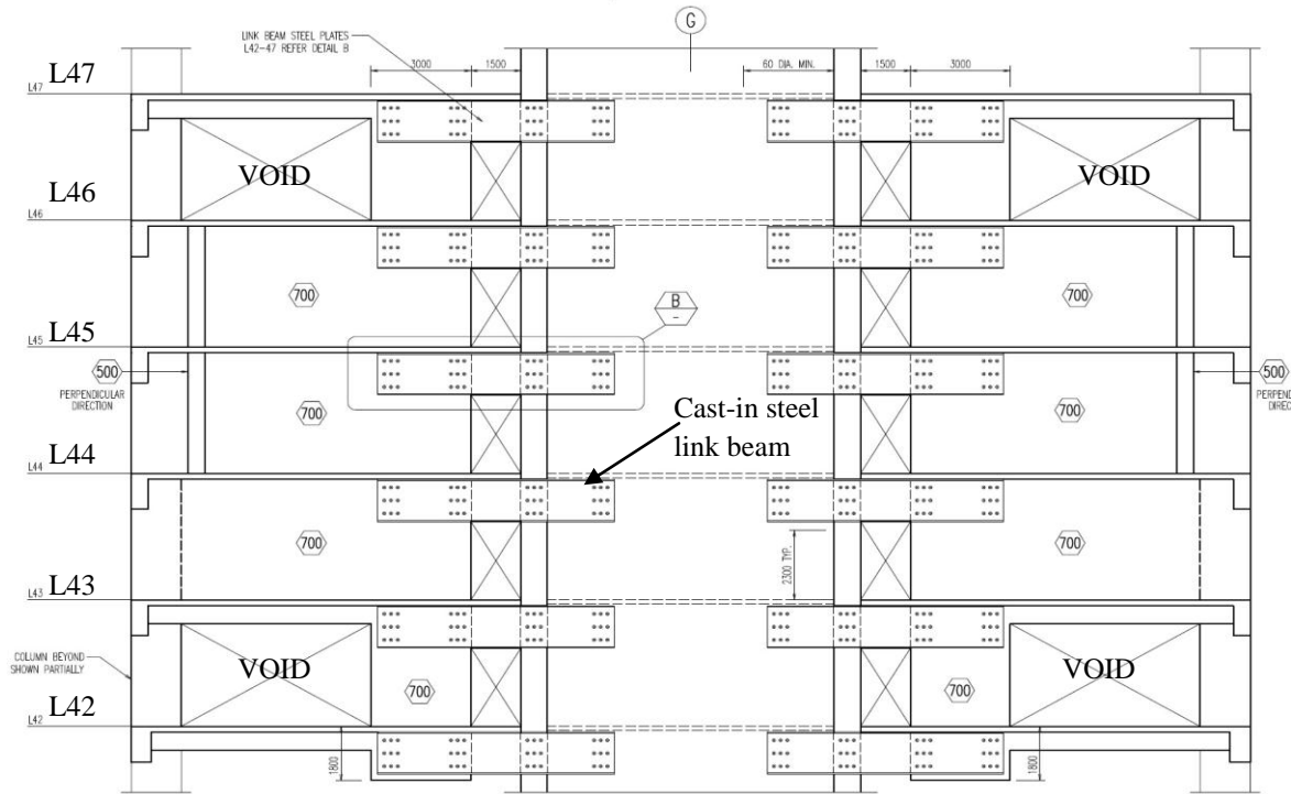
Figure 4 - Core-Outrigger Lateral System Elevation at Level 42-47 (TTW) 第 42-47 层核心支脚横向系统
