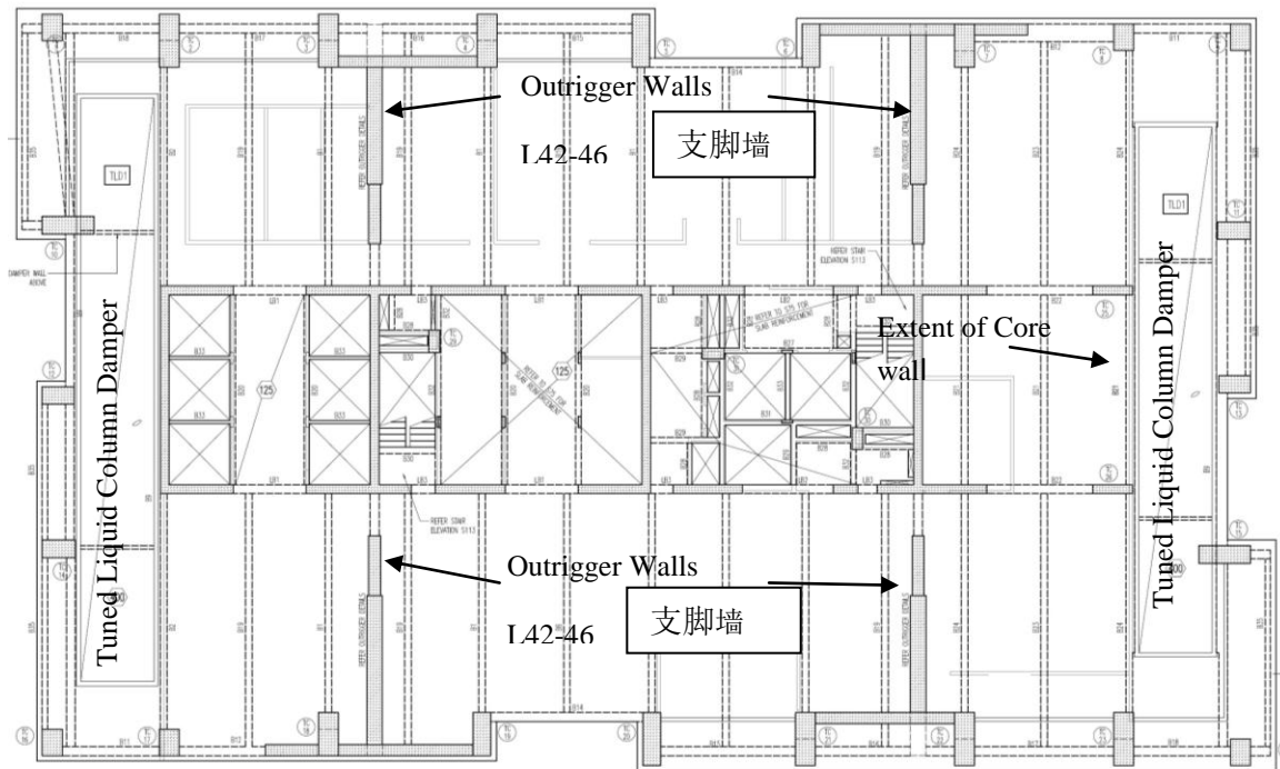
Figure 3 – Typical Floor Structure Plan 代表楼层结构平面图
